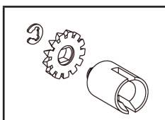
No. 505071 Roue dentée conique B diff. Differential bevel gear set
